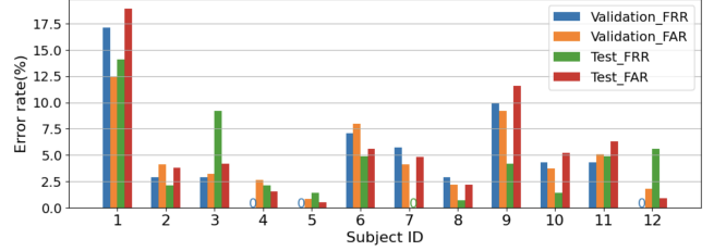
Fig. 6: Individual authentication performance with majority vote (zeros indicates the corresponding error rate is 0).
